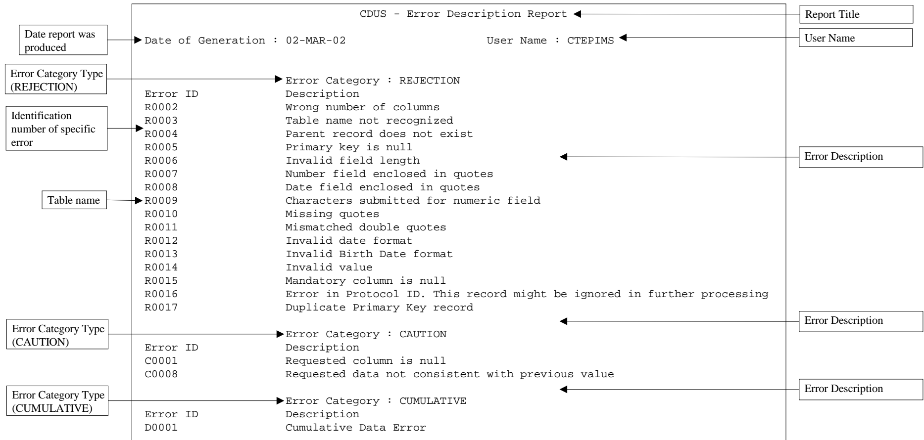
FIGURE 4: CDUS Error Description Report
